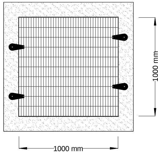
3c. Configuration of STAY GRATE™ SS5 units for 1000mm x 1000mm grate.
