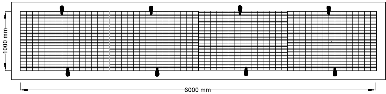
3e. Configuration of STAY GRATE™ SS5 units for 6000mm x 1000mm grate.
