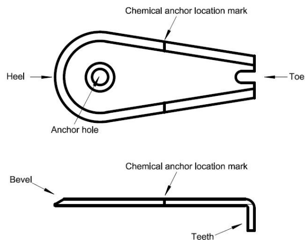
Figure 1. Plan and Profile of STAY GRATE™ SS5 unit.
