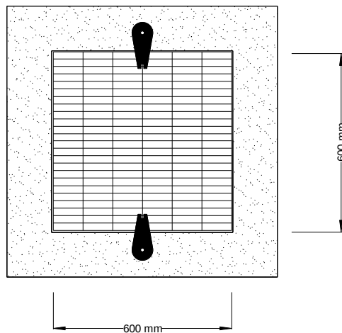
3b. Configuration of STAY GRATE™ SS5 units for 600mm x 600mm grate.
