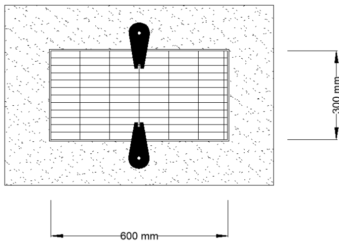
3a. Configuration of STAY GRATE™ SS5 units for 300mm x 600mm grate.
