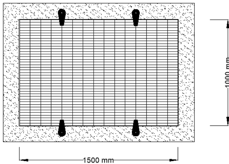
3d. Configuration of STAY GRATE™ SS5 units for 1000mm x 1500mm grate.
